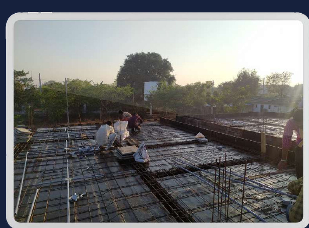
Slab Centering work
